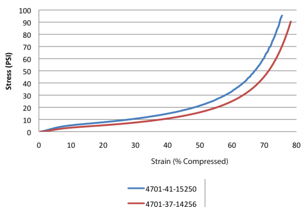
Compressibility Comparison
