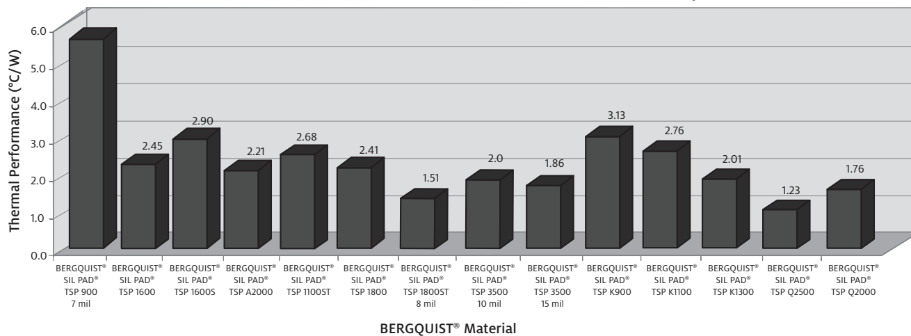
SIL PAD® Thermal Performance Overview (TO-220 Test at 50 psi)
