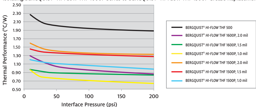
Isolating BERGQUIST® HI-FLOW THF 1600P Series to BERGQUIST® HI-FLOW THF 1500P Grease Replacement Materials
