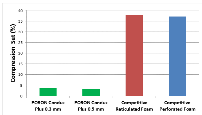
Compression Set
