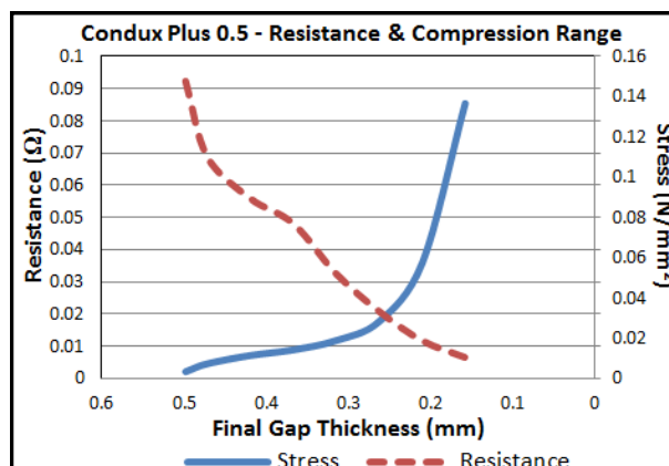
Figure 2: Condux Plus 0.5 mm Resistance & Compression
