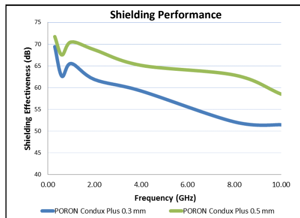
Figure 3: Condux Plus 0.3 mm & 0.5 mm Shielding Effectiveness Graph
