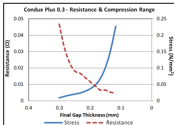
Figure 1: Condux Plus 0.3 mm Resistance & Compression
